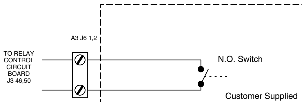
Figure 9-12 Typical Door Interlock Connection to CPDU
