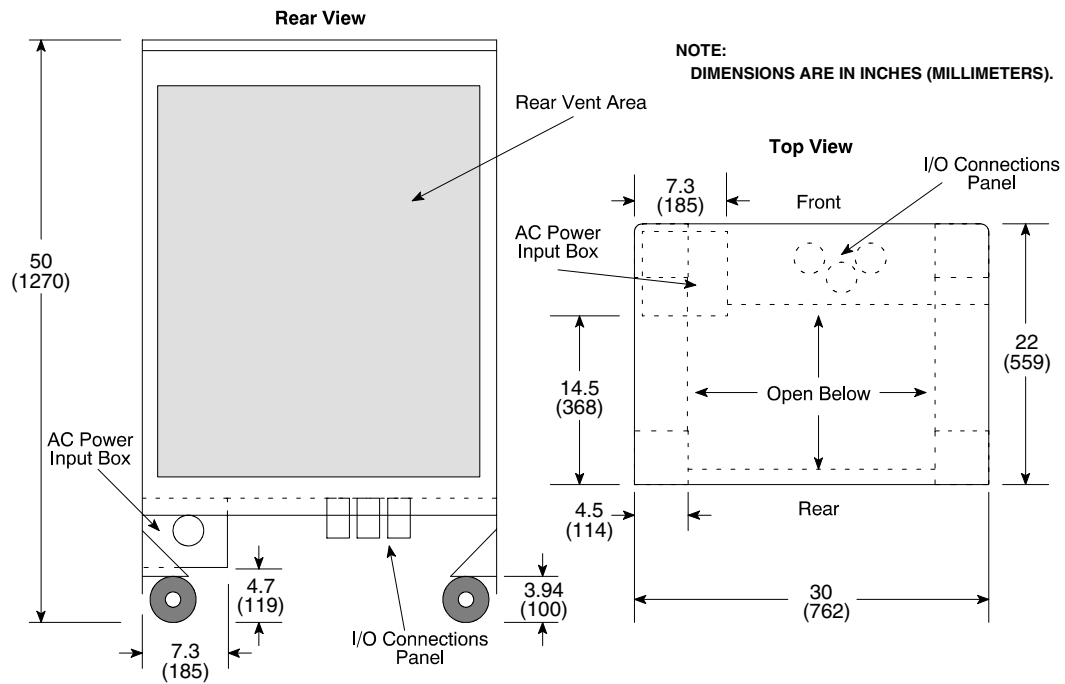
Figure 4-10 Compact Power Distribution Unit (CPDU)
