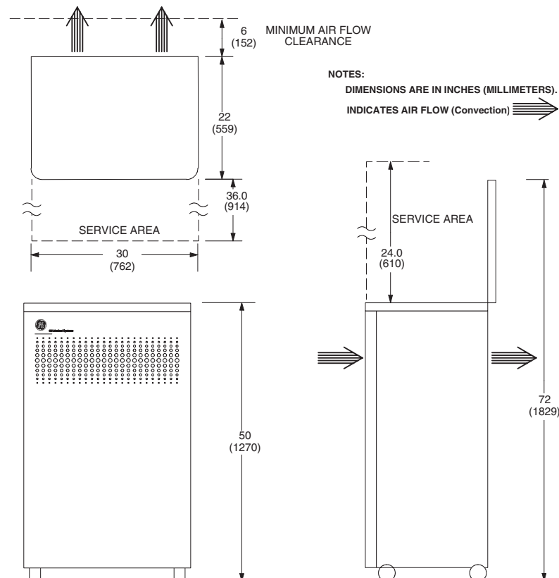
Figure 4-11 Compact Power Distribution Unit (CPDU)
