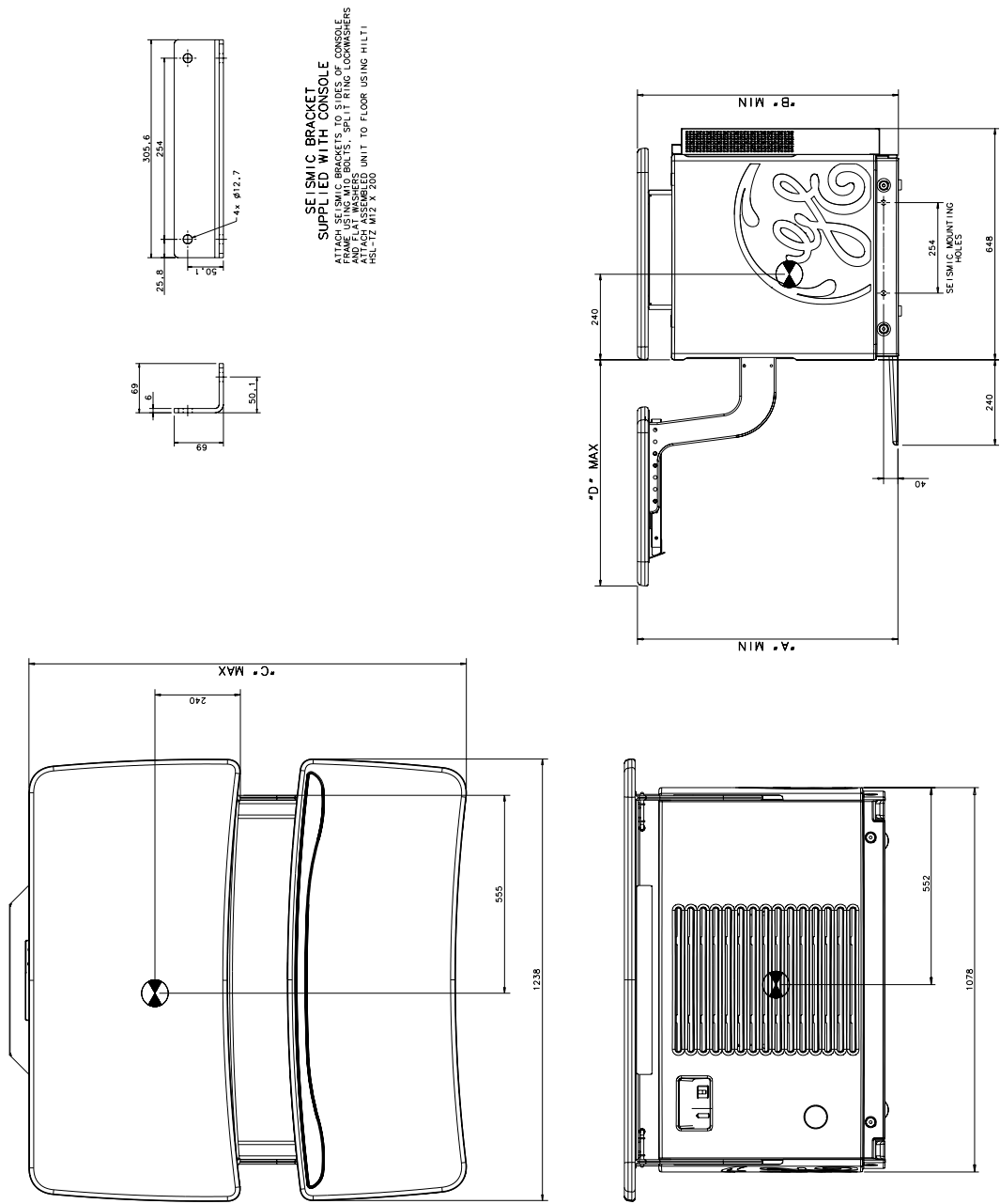
Figure 6-8 Operator's Console (Global Console)
