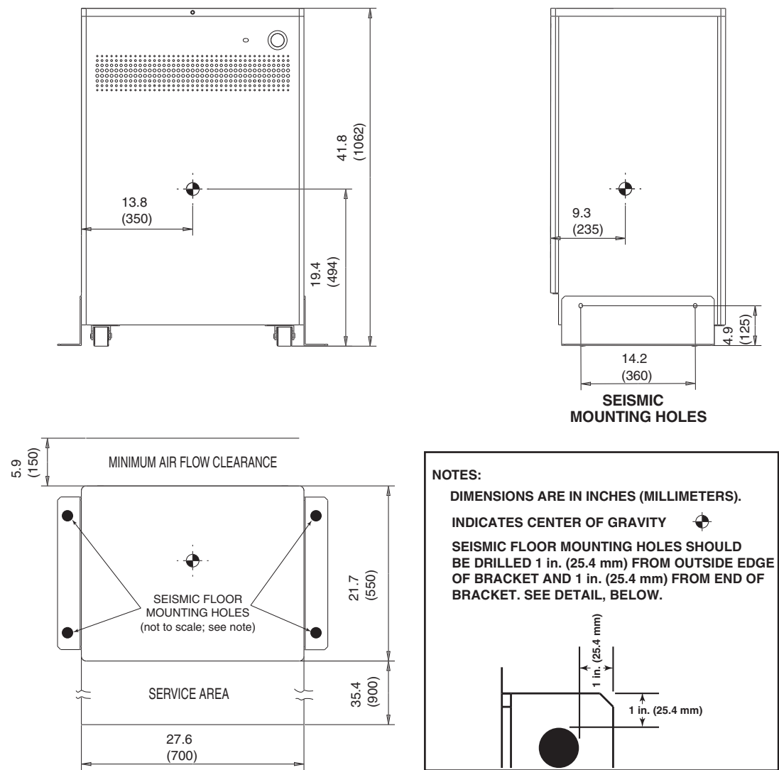
Figure 6-6 Power Distribution Unit (NGPDU)
